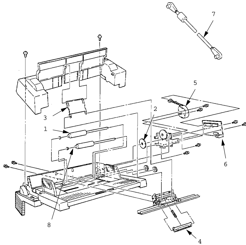
Figure 6-1 Multi-Purpose Feeder
